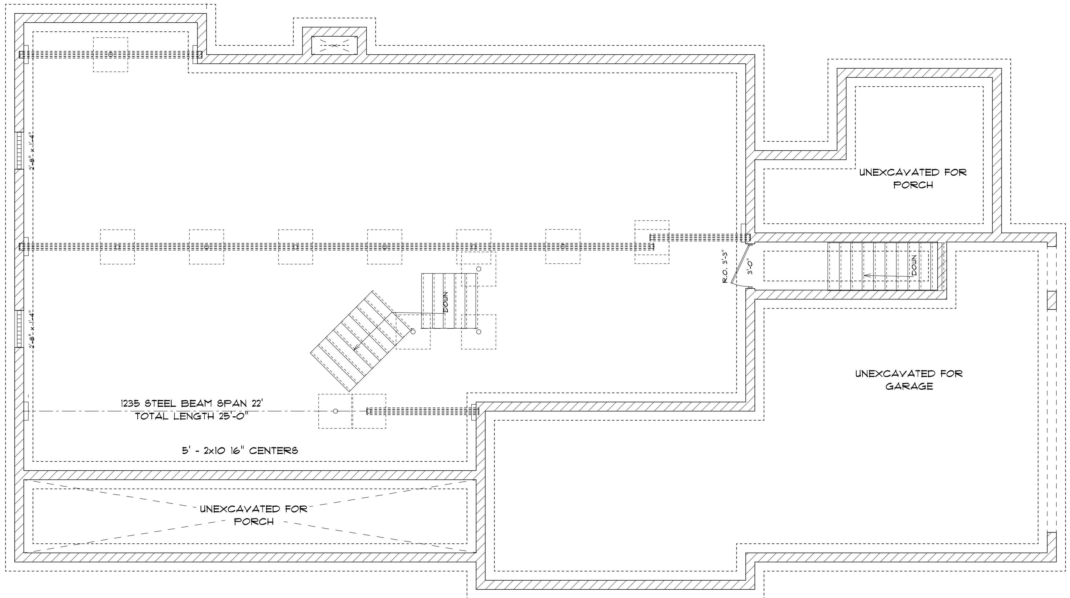
FOUNDATION PLAN
